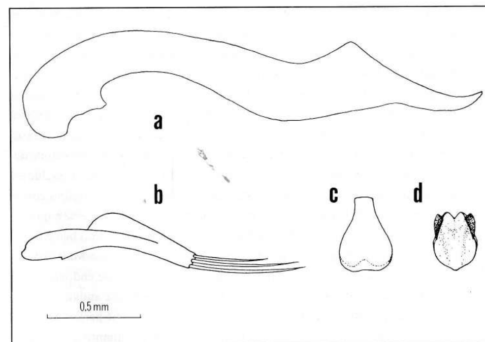
Fig. 2 - Anophthalmus mariae SCHATZM. di Costa Stretta (UD): a) edeago in visione laterale; b) paramero sinistro; c) ligula; d) lamella copulatrice. - Anophthalmus mariae SCHATZM. from Costa Stretta (province of Udine, North-Eastern Italy): a) aedeagus in lateral view; b) left paramere; c) ligula; d) copulatory piece.
