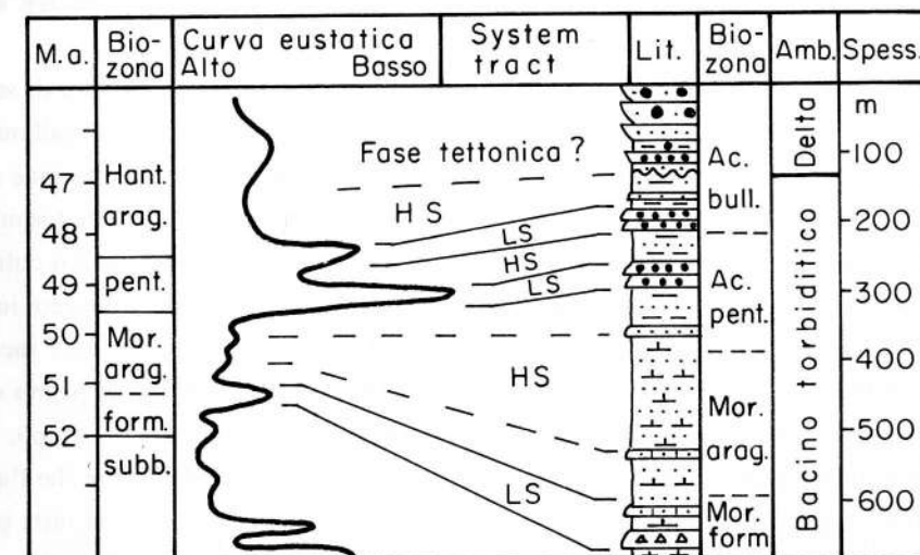
Fig. 13 - Confronto tra la curva eustatica (da HAQ et al., 1987) e la successione dei colli di Rosazzo, Rocca Bernarda e Cormons. HS = high stand; LS = low stand. - Comparison of the eustatic sea level curve (after Haq et al., 1987) with the sequence of the hills of Rosazzo, Rocca Bernarda and Cormons. HS = high stand; LS = low stand.
