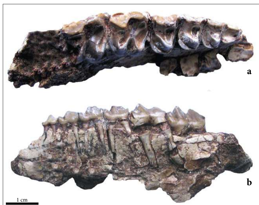
Fig. 6 - Eoletes gracilis ; the fragment of the 136 /2-08 upper jaw with P2 ÷ M3 teeth; a) occlusal view, b) buccal view.
